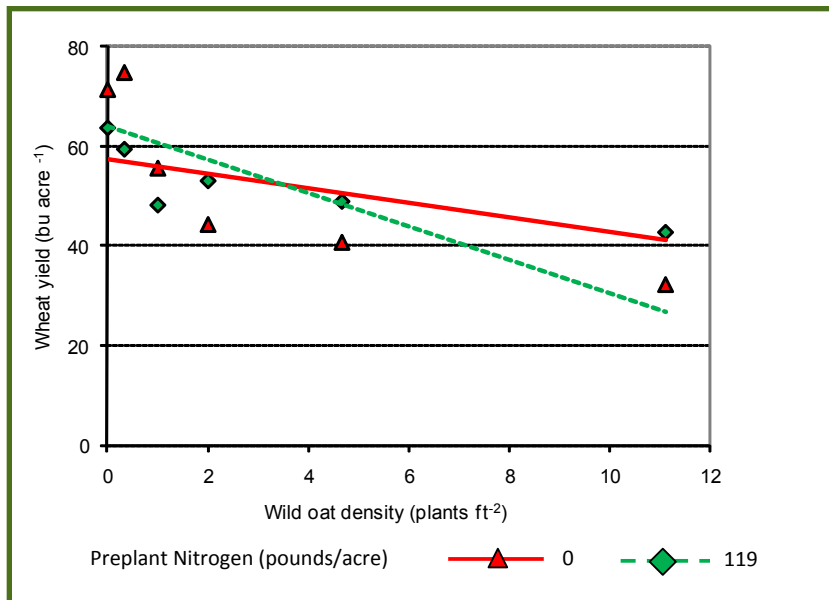
Figure 4. Impact of wild oats on wheat yield increases with nitrogen availability (Carlson & Hill, 1986)
